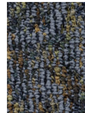
7565 Titian
